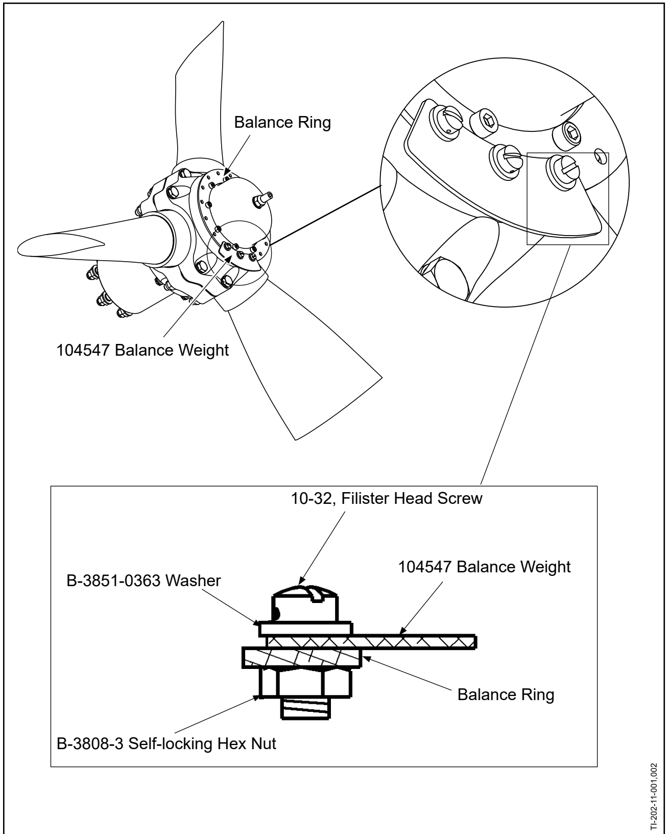
Location of Balance Weights on the Bantam Propeller Balance Ring Figure 2-7
