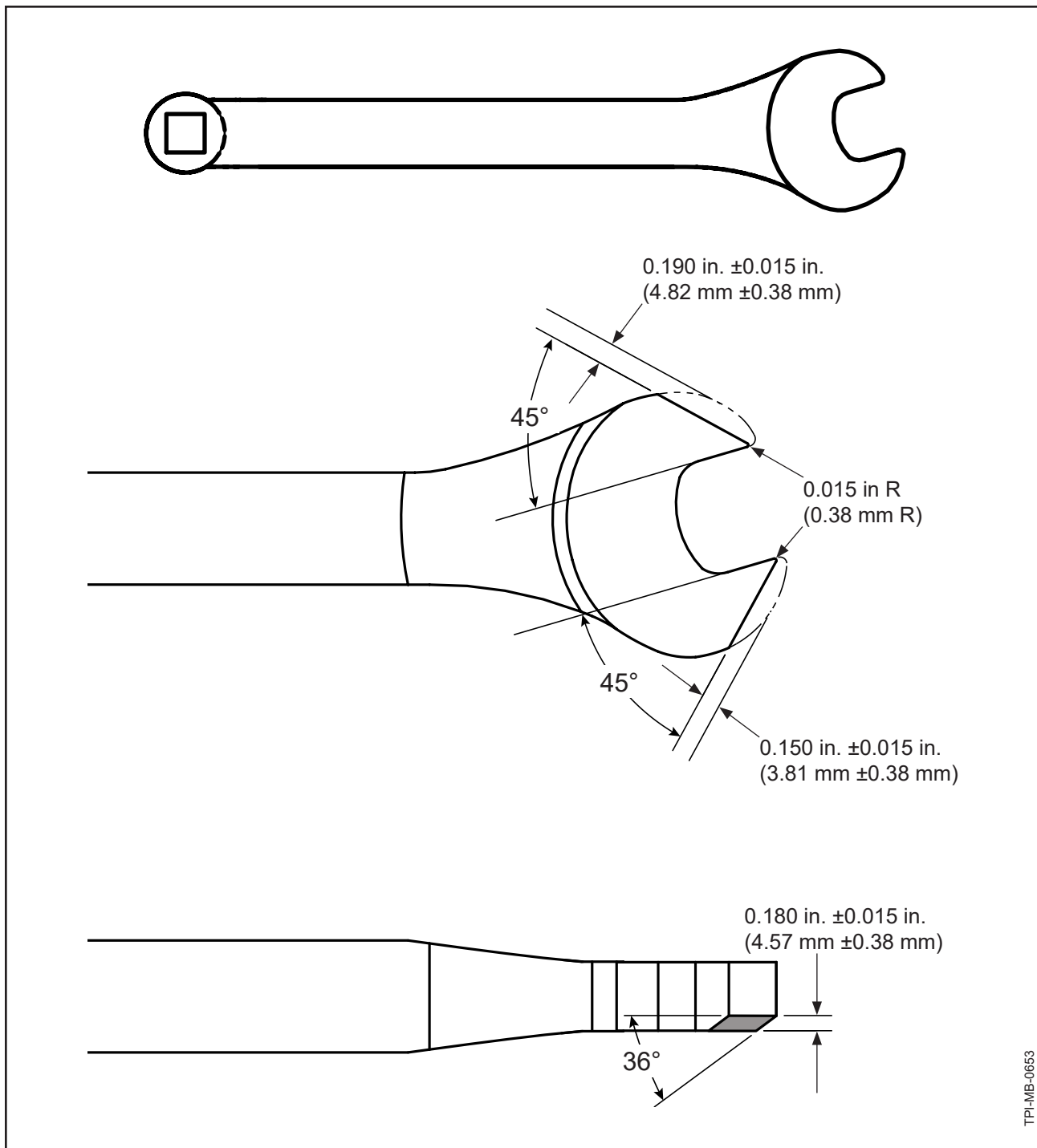
Torque Wrench Adapter Modification: Step 1 Figure 2
