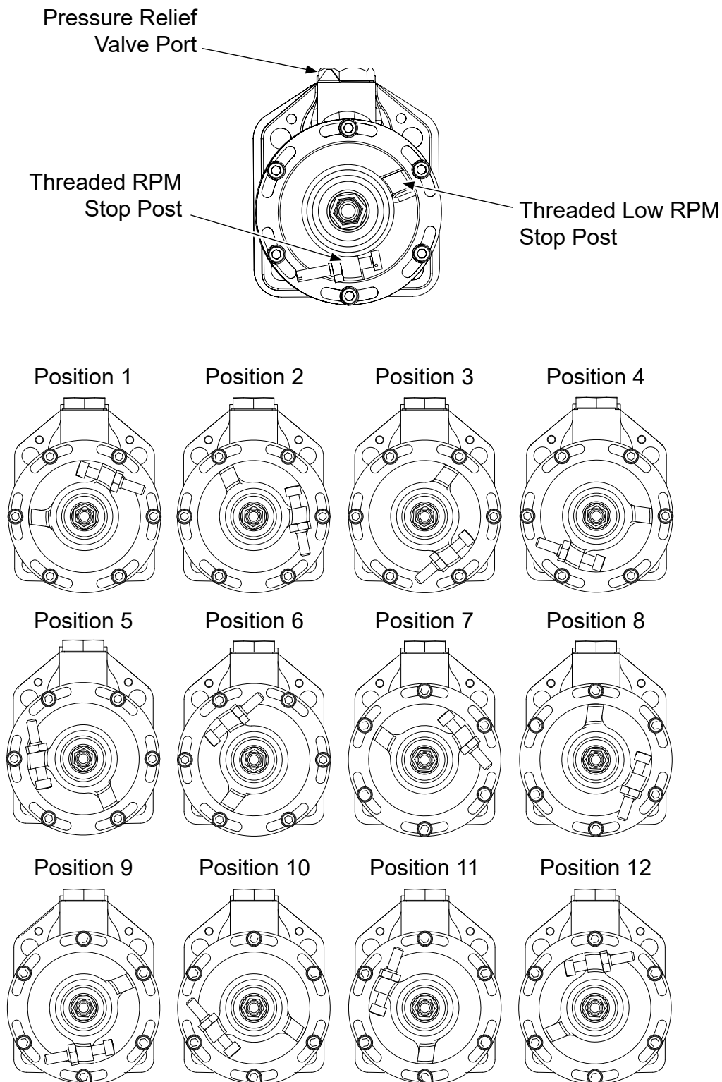
Governor Head Orientations Figure 3-6
