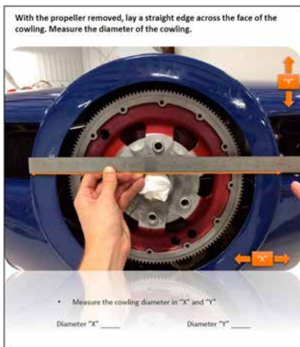
Cowling Measurement Figure 6-2
