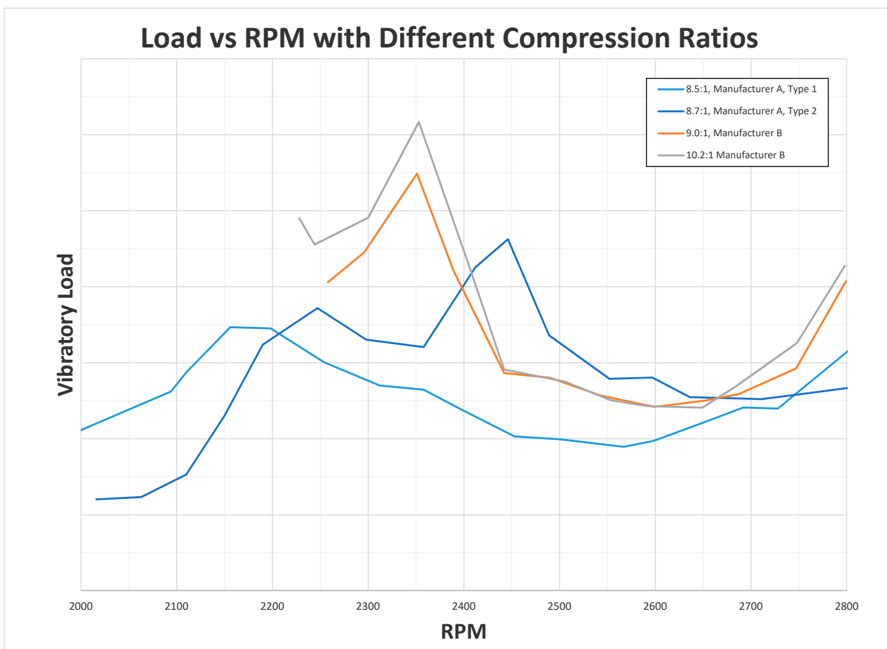
Load vs. RPM with Different Compression Ratios Figure 4-3
