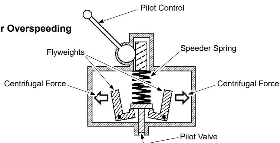
Governor Operation Examples Figure 3-3
