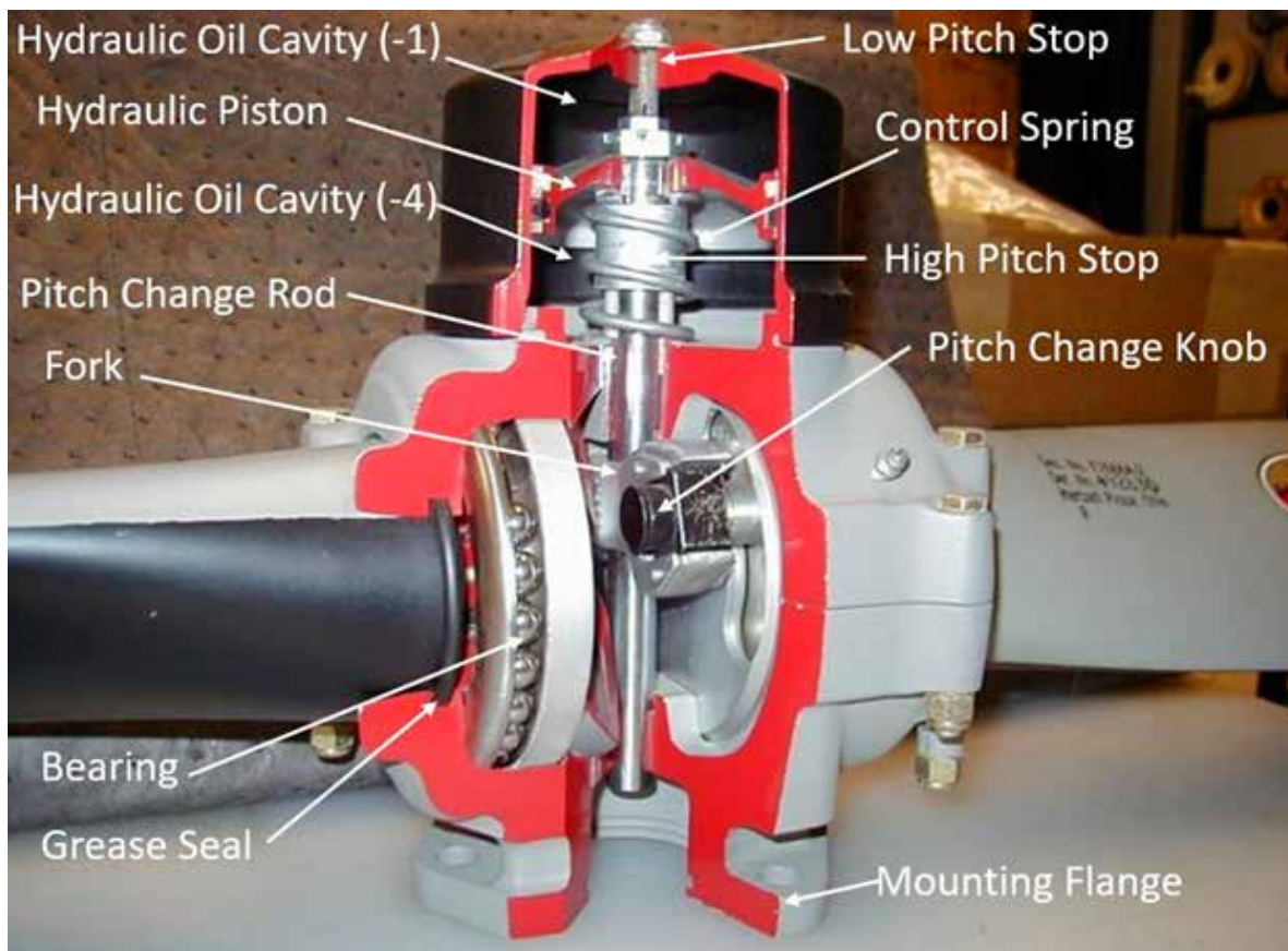
Compact Propeller: Internal Components Figure 2-1
