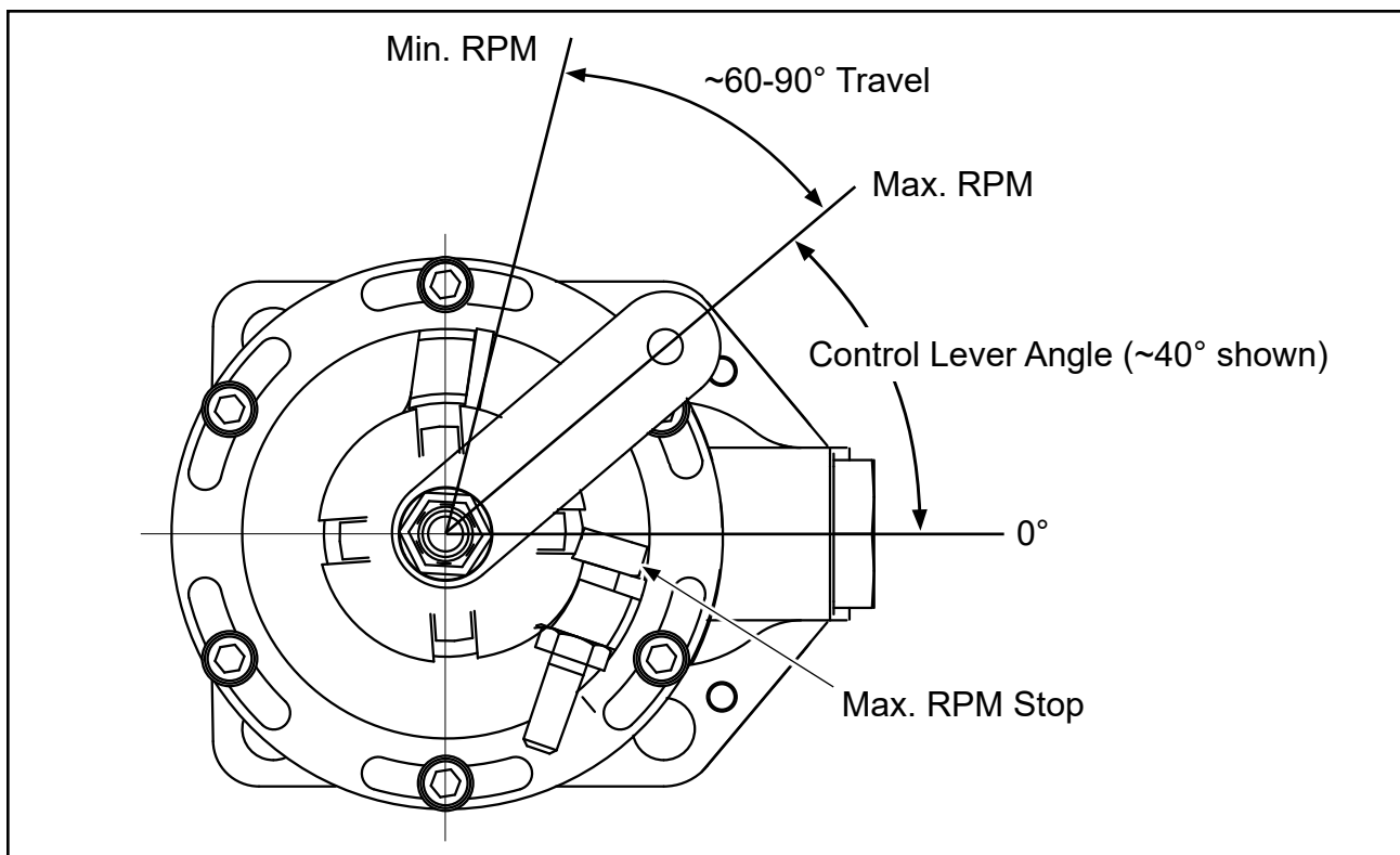
Control Lever Angle Figure 3-4
