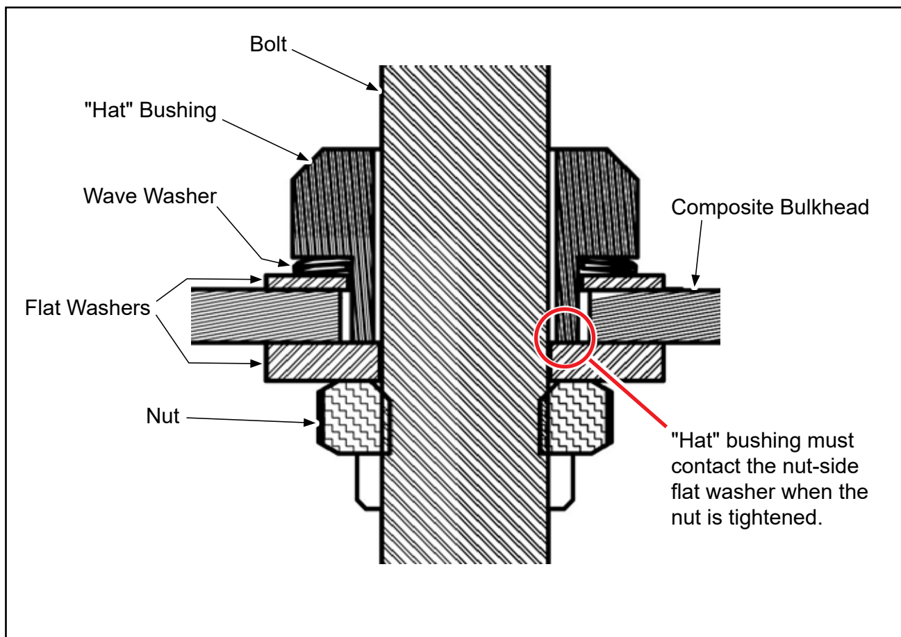
Cross-section of Spinner Mounting Hardware: Composite Bulkheads Figure 3-2
