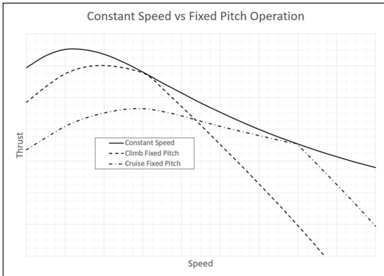
Fixed Pitch vs. Constant Speed Operation Figure 1-1
