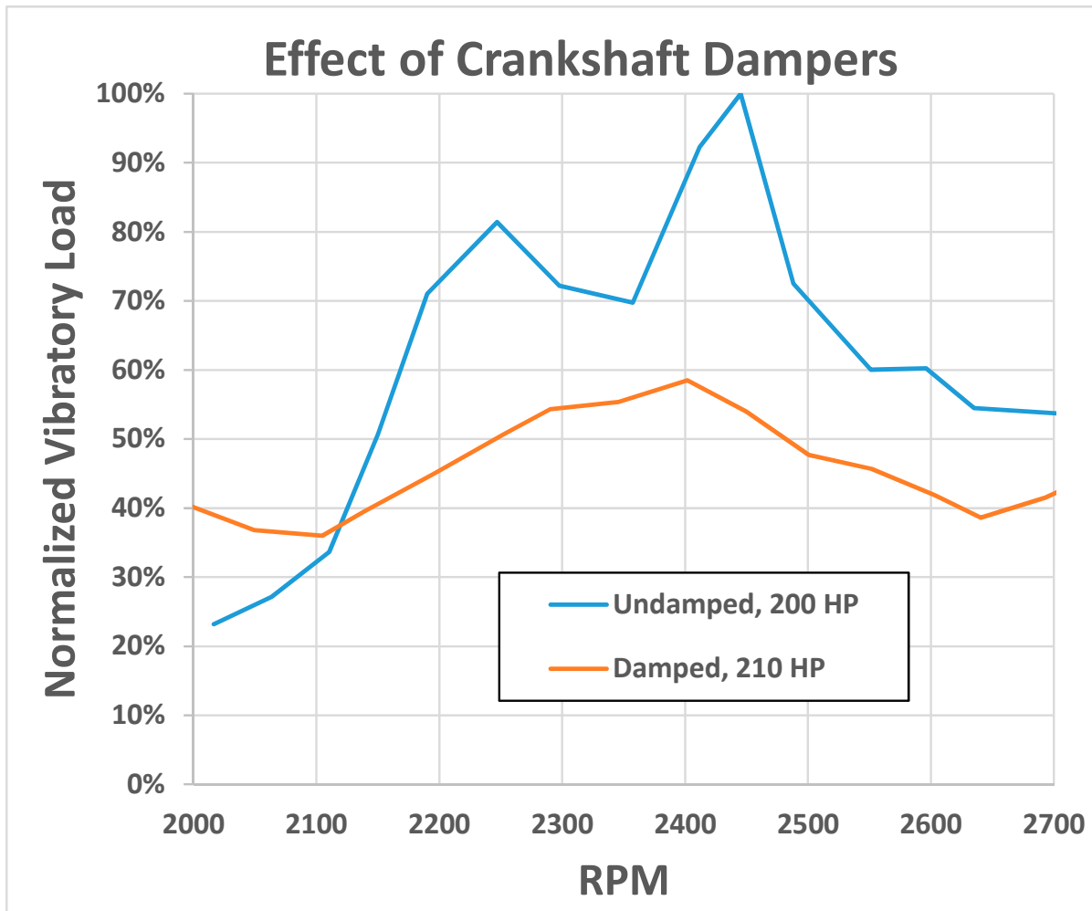
Effect of Crankshaft Dampers Figure 4-4
