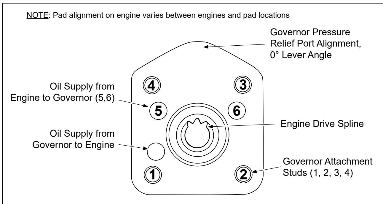
Drive Pad Figure 3-5
