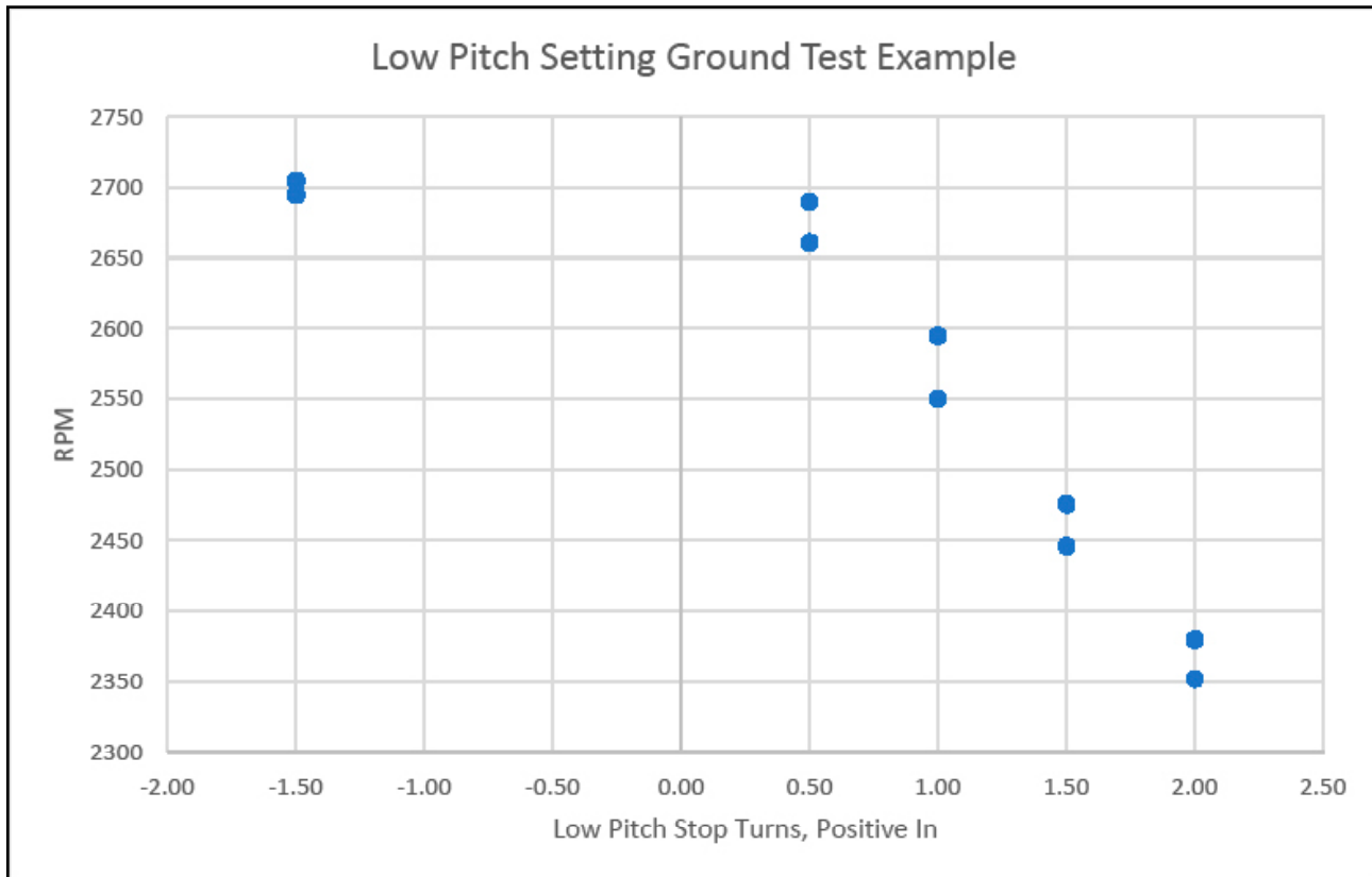
Low Pitch Setting Example Figure 6-1
