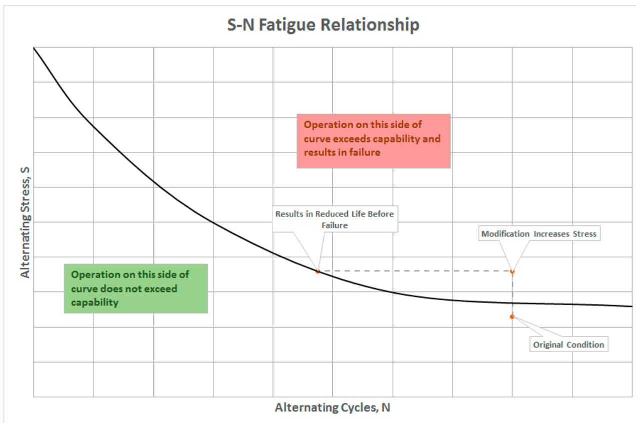
S-N Fatigue Relationship Figure 4-1
