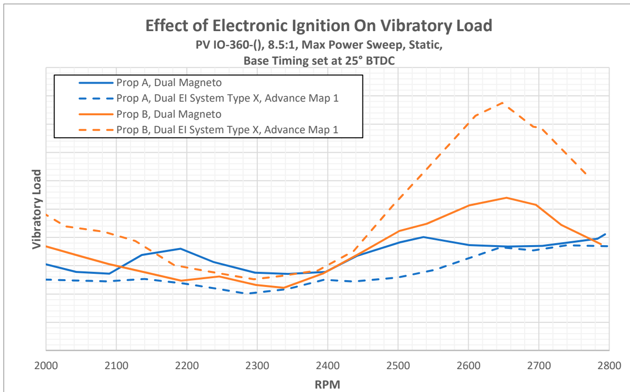
Effect of Electronic Ignition on Vibratory Load Figure 4-2
